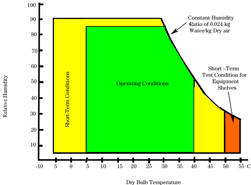
Figure 4-1 Ambient Temperature and Humidity Limits
