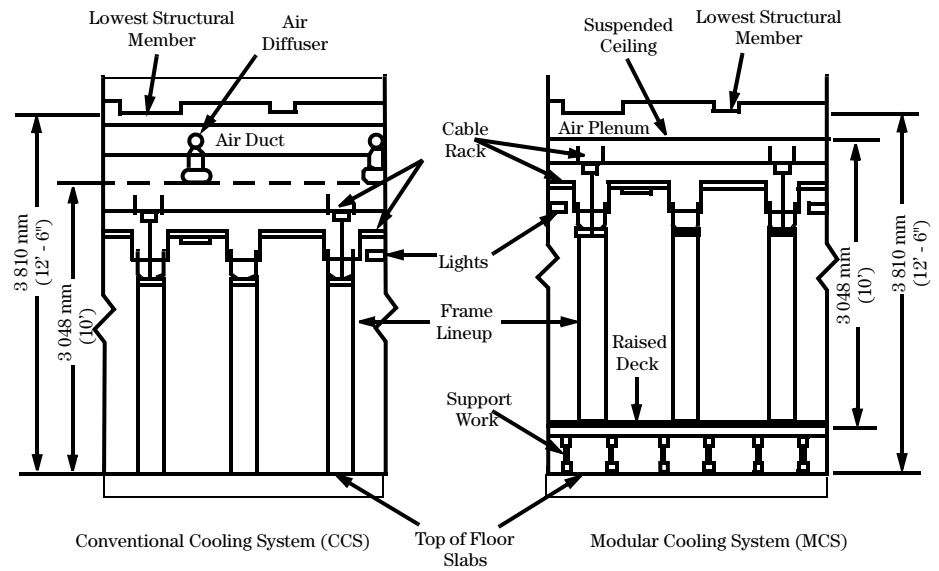
Figure 2-4 Typical Equipment Frame Area (Vertical Section)
